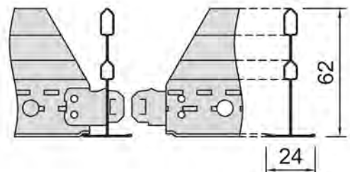
Gridline 24 MAX / Sixty2
