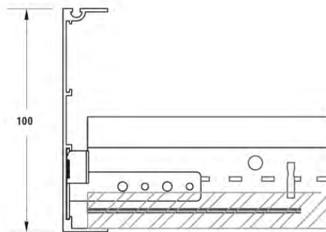
Tegular / Microlook 8 mm
